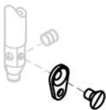
0291-000159 Thread guide 線耳 9203-312411 Screw 螺絲 (for 用於 0767-120064KH)
