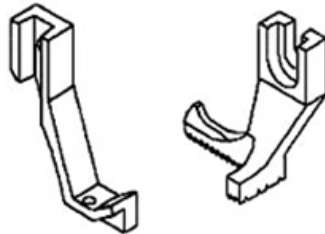
Feeding foot with right edge guide, toe on left side 右傍邊內壓腳，趾在左面
