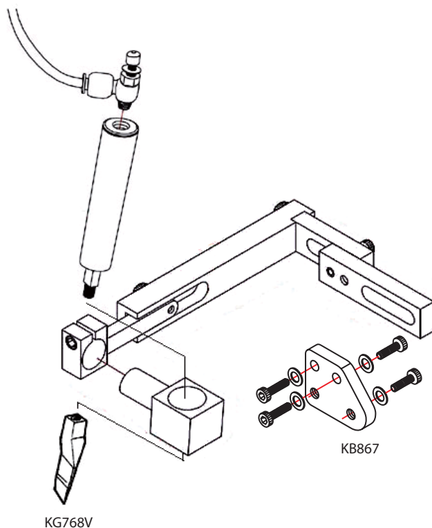
Pneumatic guiding set for 868 868 氣動傍位
