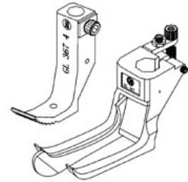
Stronger left compensating guide & wider feeding foot for HEAVY DUTY 特強左邊彈弓傍位壓腳，特闊送料
