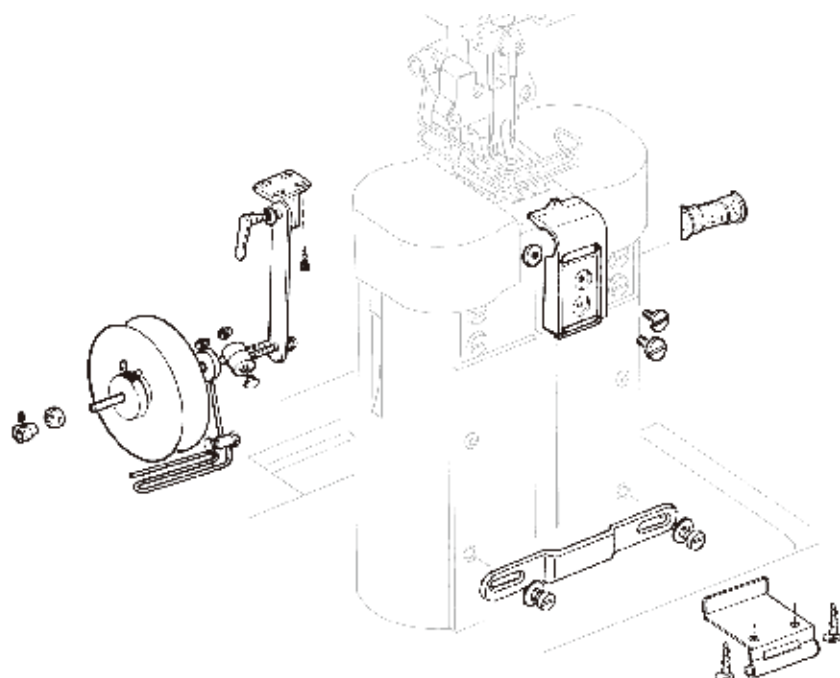
Belt guide completed set for 20mm belt 送細條套裝 (20mm)
