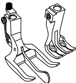
Spring type center guiding feet set 雙針中分刀壓腳
