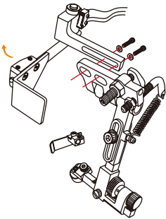
KG867 傍位連 EG-01 護目鏡 KG867 suspending guide with EG-01 eye guard
