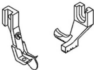
Feeding foot with right top stitch guide, toe on left side 右彈弓片傍位內壓腳，趾在左面
