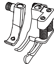
Deeper right compensating guide with balancing spring for EXTREME HEAVY DUTY 右邊彈弓傍位壓腳，超厚物用
