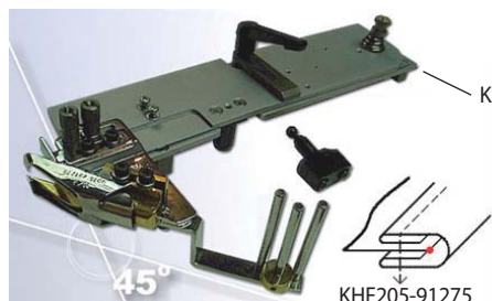
45° Moving binder, double folding 45° 可動雙環口包邊器
