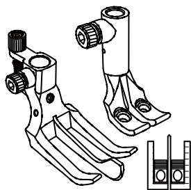
Spring type center guiding feet set 彈弓中分刀雙針壓腳
