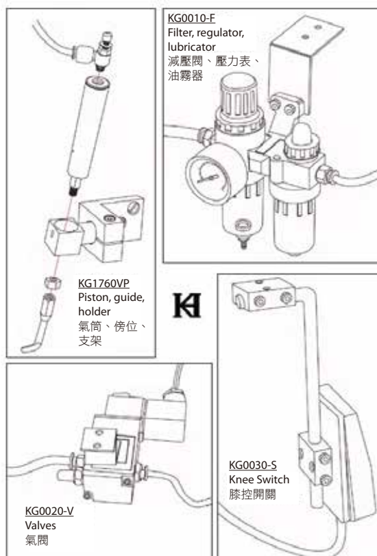
Pneumatic guide set with F.R.L. unit, knee switch and valves for Juki PLC-1760 重機PLC-1760 氣動傍位連 F.R.L. 聯組、氣閥、膝控開關
