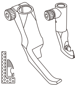
Right cording feet set 右單邊壓腳
