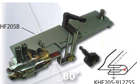
Support sheet 80° Moving binder, double folding 包邊器連接板 80° 可動雙環口包
