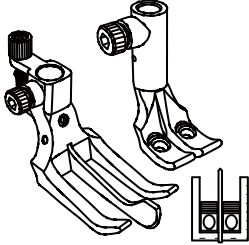
Spring type center guiding feet for 12mm stitch length 彈弓中分刀外壓腳，適合 12mm 行程用
