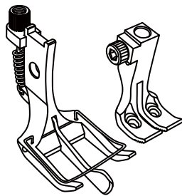
Spring type center guide feet set 彈弓中分刀壓腳
