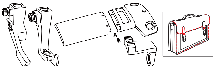
Right guiding gauge set for 205-370 205-370 右傍針位
