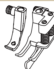
Deeper right compensating guide with balancing spring for EXTREME HEAVY DUTY 右邊彈弓傍位壓腳，超厚物用
