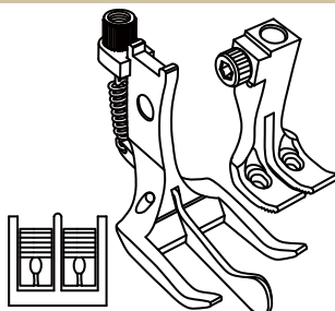
Spring type center guiding feet 彈弓中分刀雙針壓腳
