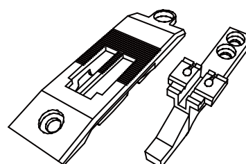
Needle plate & feed dog for 1246 with thread trimmer 1246 剪線用針板/送布牙
