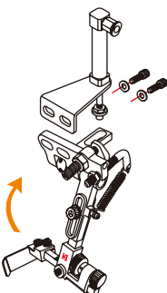
Pneumatic lifted edge guide for universal machines 泛用型氣動升降傍位
