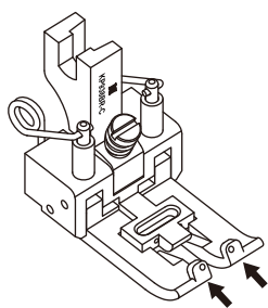
針孔尺寸 Needle hole size: 8mm x 2mm
