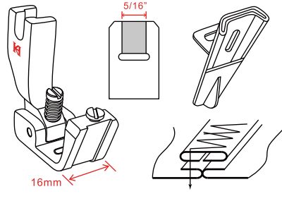
開式縫面貼壓腳 (附中央導向片) Open seam tape attaching foot (with center guide)
