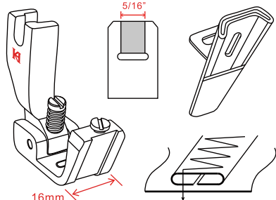
面貼壓腳 Tape attaching foot
