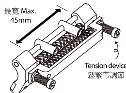
導帶滾輪 (連鬆緊帶調節) Roller guide (with tension device)
