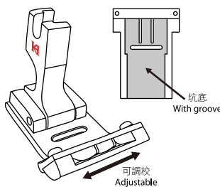
導帶落坑導傍壓腳 Guiding foot with groove
