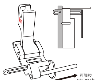
導帶壓腳 Guiding foot
