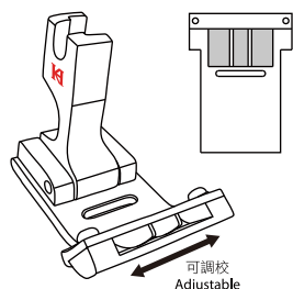
導帶坑面貼壓腳 Grooved tape attaching foot
