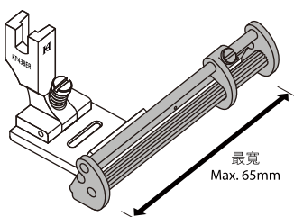
導帶滾輪壓腳 Roller guiding foot
