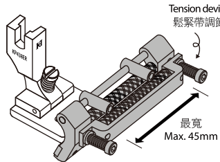
導帶滾輪壓腳 (連鬆緊帶調節) Roller guiding foot (with tension device)
