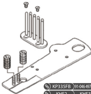
Arm cover for binding 包邊筒架
