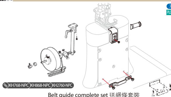
Belt guide complete set 送細條套裝
