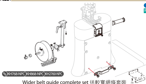
Wider belt guide complete set 送較寬細條套裝
