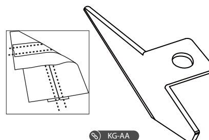
(Improved version of 0667-245004) (0667-245004 改良款式) Seam middle guide 中分傍刀
