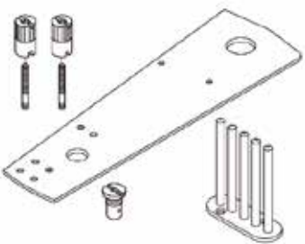
Arm cover for binding on DA69 machine 杜克普69用包邊筒架
