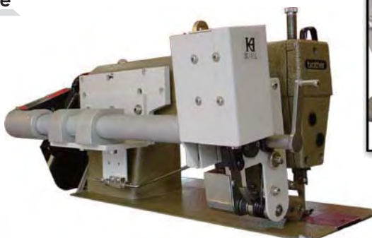
SU-91L 單針平縫電動提升拖輪 Puller for 1-needle machine with Lifting Device
