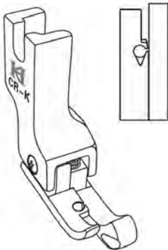
CR-K Right Compensating Feet for Thin/ Knitting Material 右高低壓腳 (薄物及針織物用)
