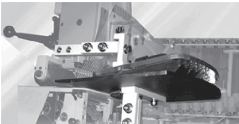
Presser feet & Center Slice for KHF1412-PTVB KHF1412-PTVB 用壓腳和分中片
