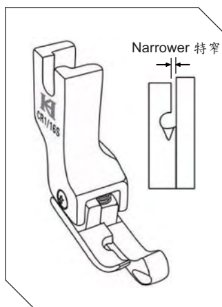
CR-S Right Compensating Feet for Thin/ Knitting Material 右高低壓腳 (薄物及針織物用)
