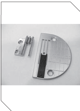
APS-10 Needle Plate for Anti-Puckering 防皺縮針板
