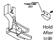
P35GK Standard Feet with Needle Guard and Thread Cutter 標準壓腳 (連護針罩及割線刀)
