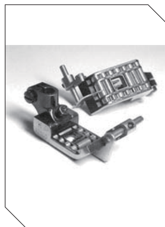
R2500 Chainstitch Roller Feet 繡縫車滾輪壓腳
