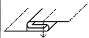
KHF 102 Single Needle Lap Seam Attachment (part 2/2) 單針接袖器(第二部份)
