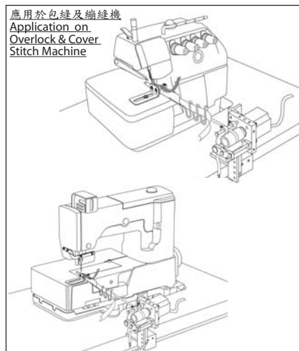
KHF 150 (Tailor-made) Spaghetti Attachment 通心暗線縫拉帶器
