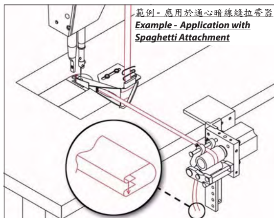
Feed Downward 向下送料
