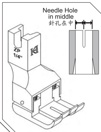
ZP Double Compensating Feet 左右高低壓腳 Case 1
