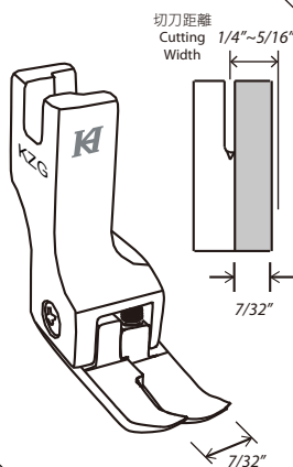
KZG 襯衫切下級領壓腳 Collar Band Trimming Foot
