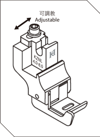
KZN-L 左傍刀 (可調教) 壓腳 Adjustable Left Guide Foot
