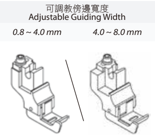
KZN-L 左傍刀 (可調教) 壓腳 Adjustable Left Guide Foot
