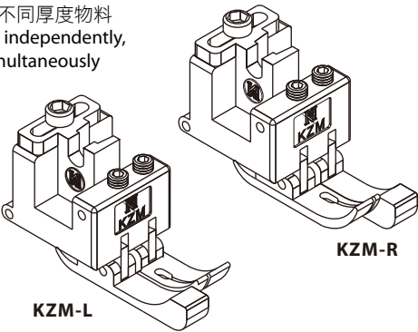
KZM-R 右導傍高低壓腳 (壓力可調教) Right Compensating Foot (Presser Adjustable)
