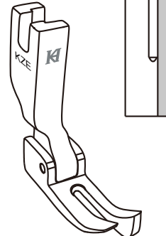
KZE 襯衫右傍口領壓腳 Upper Collar Coverstitch Foot with Right Guide
