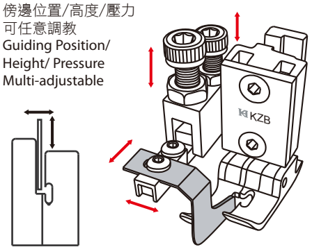
KZB 平車傍邊間線壓腳 Mult-adjustable Guiding Foot 傍邊位置/高度/壓力可任意調教 Guiding Position/ Height/ Pressure Multi-adjustable
