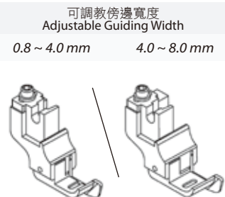
KZN-R 右傍刀 (可調教) 壓腳 Adjustable Right Guide Foot
